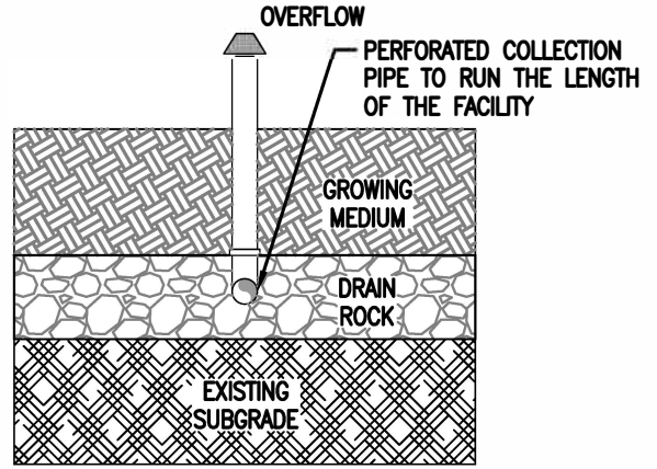
HYBRID STORMWATER HIERARCHY CATEGORY 2 OVERFLOW DIRECTED TO DRAIN ROCK. (SEE SW-251 AND SW-252 FOR MORE INFORMATION) PAC CONFIGURATION E, F
