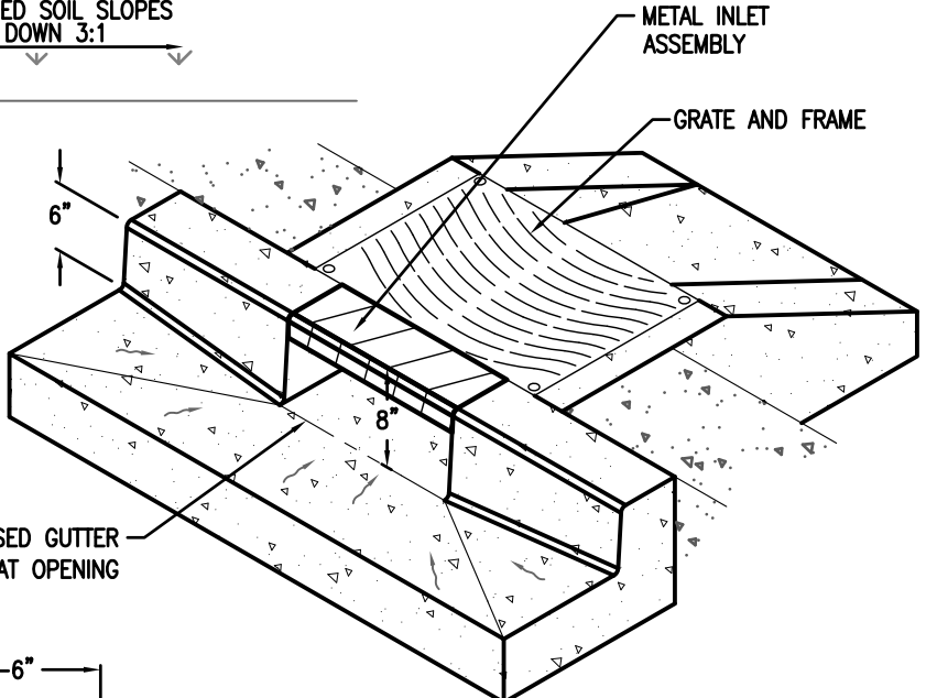
ISOMETRIC
