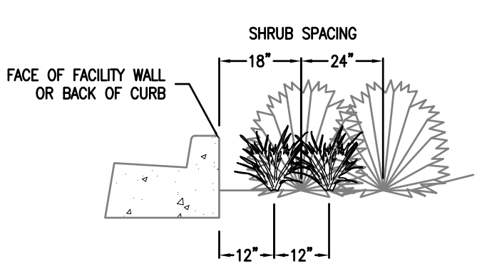
STREET SIDE OF FACILITY ELEVATION VIEW
