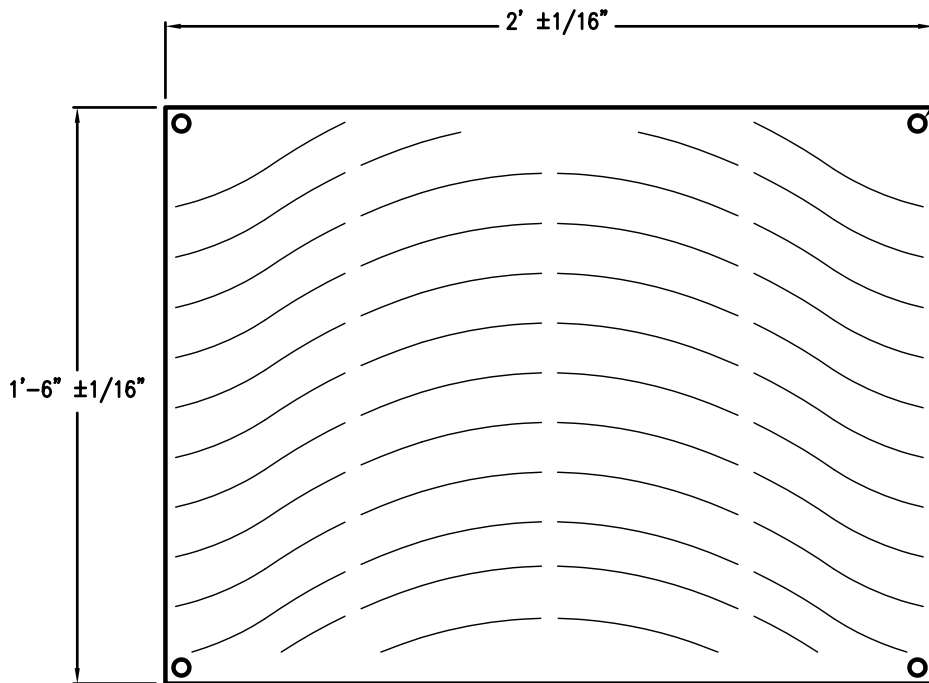
TRENCH GRATE
